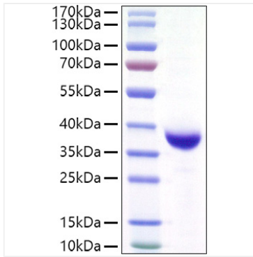
Recombinant SARS-CoV-2 Spike RBD(Lambda/C.37) Protein was determined by SDS-PAGE under reducing conditions with Coomassie Blue.
