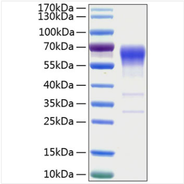
Recombinant Human Activin RIIB/ACVR2B Protein was determined by SDS-PAGE with Coomassie Blue, showing a band at 50-70 kDa.
