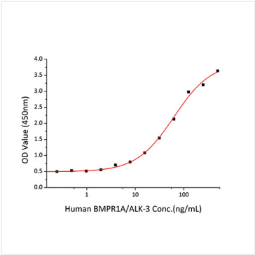
Immobilized Human ACVR2B at 1 µg/mL (100 µL/well) can bind Human BMPRI1A with a linear range of 0.5-62.5 ng/mL.
