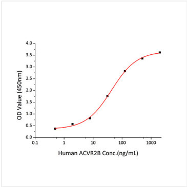
Immobilized Human CD105 at 1µg/mL (100 µL/well) can bind Human ACVR2B with a linear range of 0.49-43.03 ng/mL.
